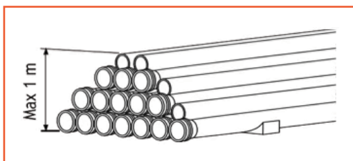
STOCCAGGIO TUBI | STORAGE OF PIPES ON THE STOCKS
